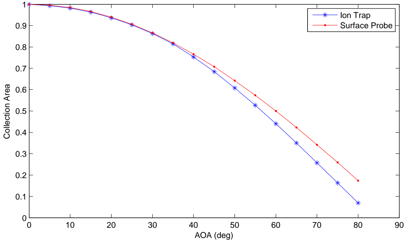
PLP Ion Trap and Surface Probe effective collector area.
